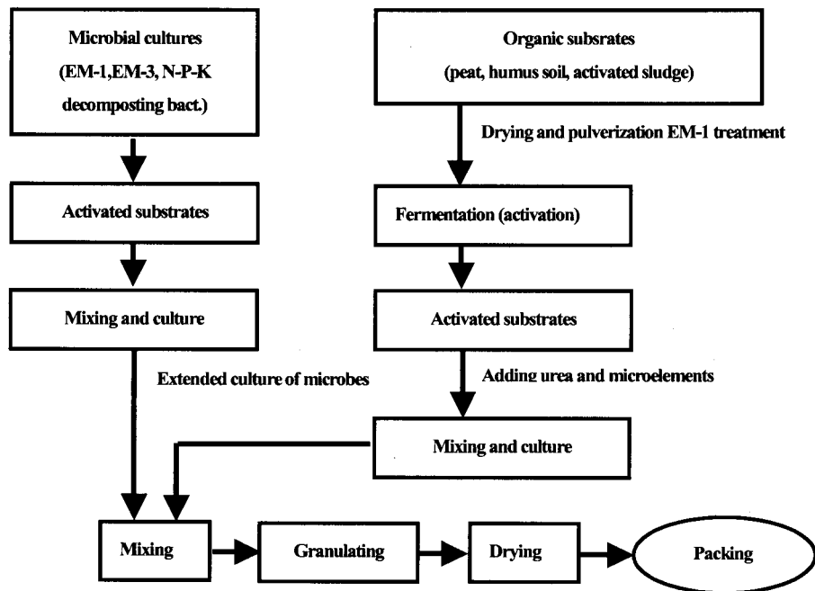
Figure 2. Manufacturing Process of Multi-ingredient Compost
